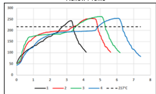
Reflow Profile
